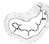
Figure 11. Retinal photoisomerization dynamics. Bottom-left: transformation from cis to trans -2-butene; bottom-right: suggested constraints on retinal in protein rhodopsin (adapted from Refs. [19,20]).
