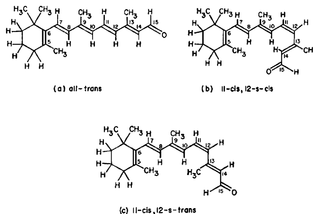
Semiclassical trajectory approach to photoisomerization
